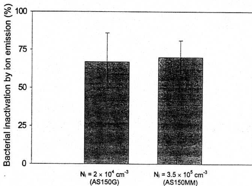
Figure 8: Bactericidal effect of ion emission by two air ionizers on viable airborne Pseudomonas fluorescens ( t_{\text{exp}} \approx 1 \text{ min} , \text{RH} = 17 \pm 5\% ).
