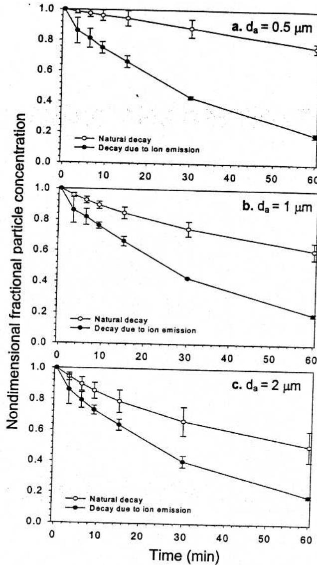
Figure 5: Non-dimensional fractional particle concentration in the large walk-in chamber ( 24.3 \text{ m}^3 ) as measured by the ELPI. Decay due to ion emission represents the data obtained with AS150MM and smoke particles.
