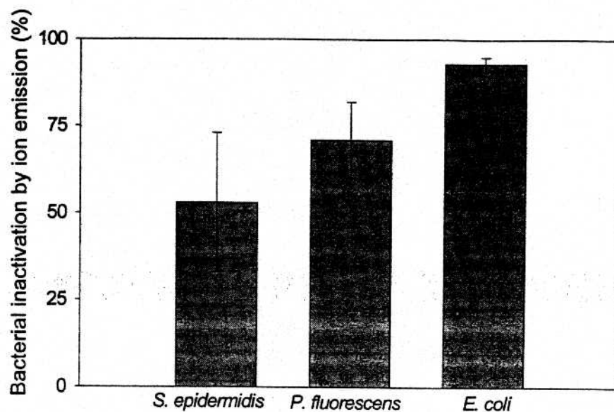
Figure 7: Bactericidal effect of ion emission by AS150MM on viable airborne microorganisms ( N_i = 3.5 \times 10^5 \text{ cm}^{-3} , \text{RH} = 17 \pm 5\% , t_{\text{exp}} \approx 1 \text{ min.} ).
