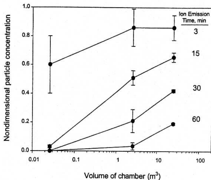
Figure 6: Non-dimensional particle concentrations as a function of the volume of the test chamber and the time of ion emission by AS150MM (data integrated within the particle size range of 0.5 – 2.0 \mu\text{m} ).
